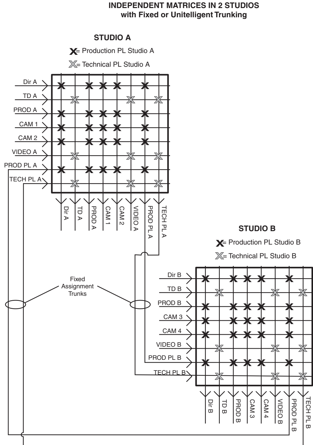
Figure 1.3 Fixed Trunking
