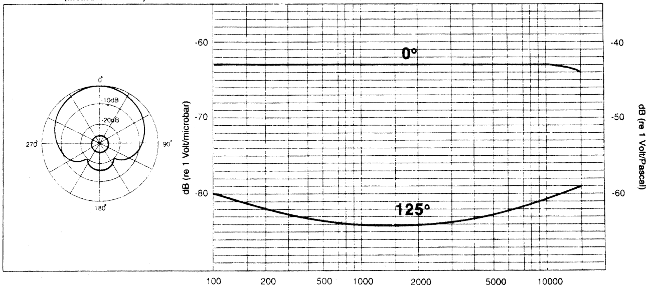
FREQUENCY RESPONSE (Measured free field at 1m with standard preamplifier, 1.3V supply and high impedance amplifier.)
