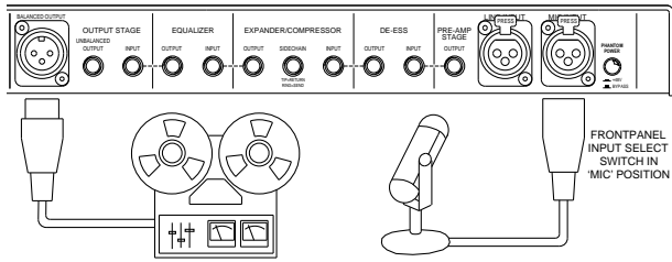
Figure 7-2. Hookup for standalone operation.
