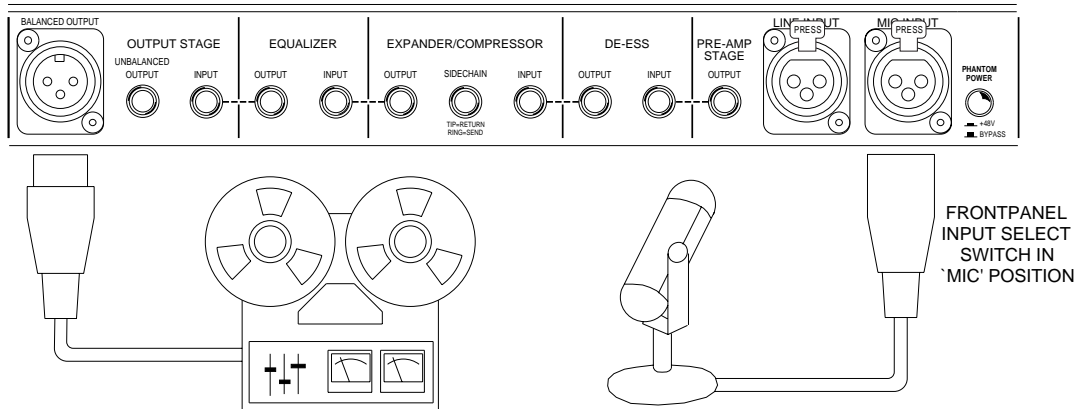
Figure 7-2. Hookup for stand-alone operation
