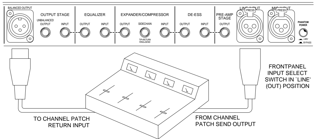
Figure 7-3. Using the 528E as a channel insert device
