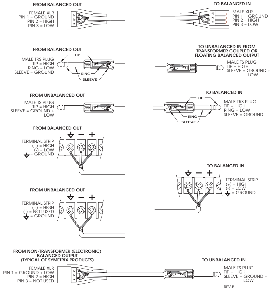
Figure 9-1. Input and output connector wiring. These diagrams represent the majority of connectors used in modern audio equipment. Locate the source connector in the left column and match it up with the destination connector in the right column. Wire your cable according to the diagrams.
