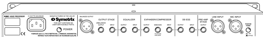
Rear panel
