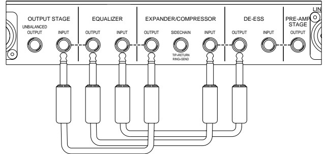
Figure 7-5. Changing the sequence of processing
