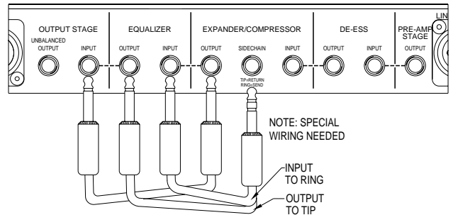
Figure 7-6. Using the equalizer in the dynamics processor's sidechain
