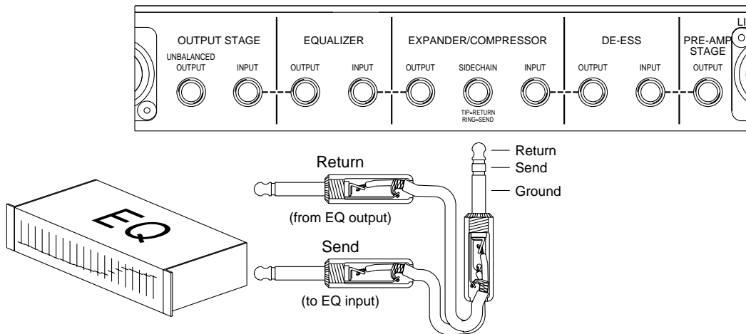
Figure 9-2. Sidechain insert jack connections
