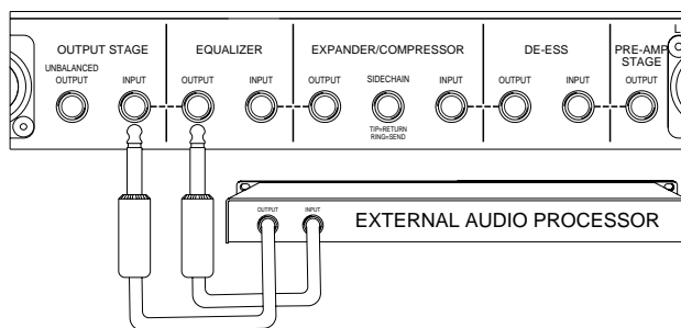
Figure 7-4. Inserting additional processing
