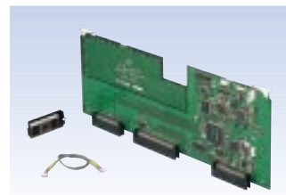
DSBK-190 i.LINK/DV Input/Output Board
