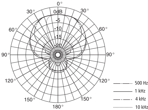
Directivity Characteristics
