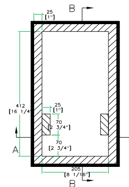
TOP VIEW OF COVER
