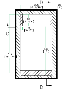
TOP VIEW OF BASE
