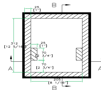
TOP VIEW OF COVER
