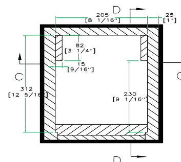
TOP VIEW OF BASE
