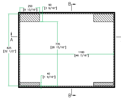
TOP VIEW OF COVER
