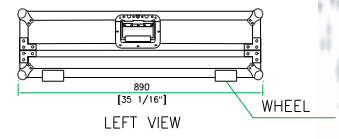
LEFT VIEW
