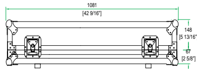
BACK VIEW
