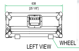
LEFT VIEW
