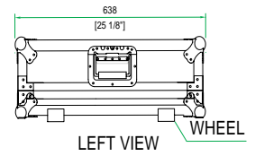
LEFT VIEW
