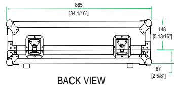
BACK VIEW
