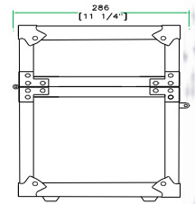
LEFT VIEW
