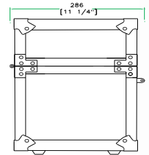
RIGHT VIEW
