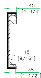
E-E VIEW
