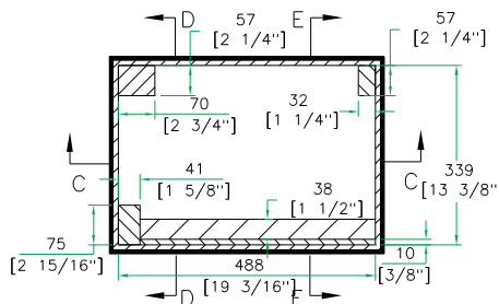
TOP VIEW OF BASE
