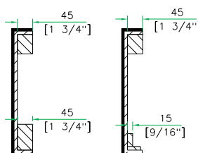
D-D VIEW
