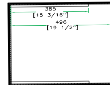
D-D VIEW
