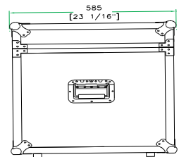
LEFT VIEW
