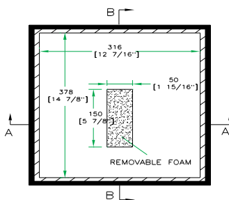
TOP VIEW OF COVER
