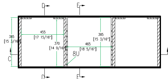
TOP VIEW OF BASE
