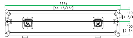
BACK VIEW
