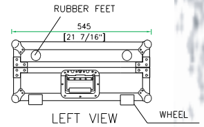
LEFT VIEW
