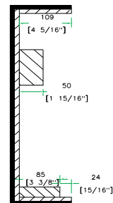
B-B VIEW
