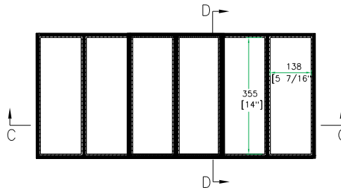
TOP VIEW OF BASE
