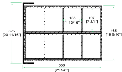
TOP VIEW OF DRAWER
