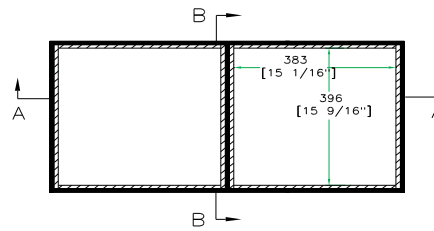
TOP VIEW OF COVER
