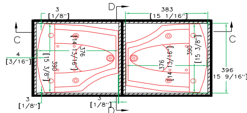
TOP VIEW OF BASE
