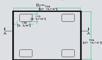
TOP VIEW OF COVER
