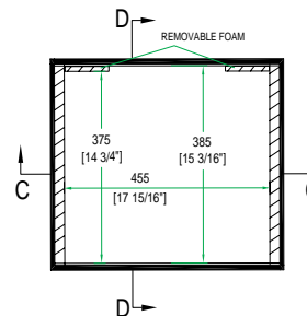
TOP VIEW OF BASE
