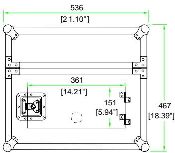
BACK VIEW
