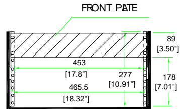
INSIDE VIEW
