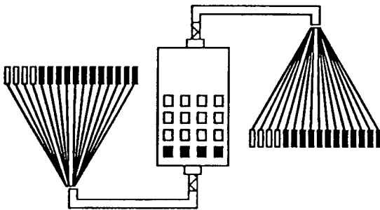
HMDX XFP/XMP- XMC/XFC Parallel XMC/XFC (Mics w/ XLR Returns)
