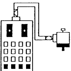
HMBTX-2 XFP/XMP-M/MPC (2) Parallel O/P M/MPC (Mics w/ XLR Returns)
