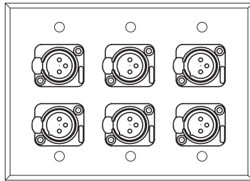
WP 3002 (6) NEUTRIK NC3FDL-1 "D-SERIES" 3 COND. LATCHING FEMALE XLR
