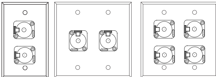
WP 1007 (2) NEUTRIK NJ3FP-6C "D-SERIES" LATCHING 3 COND(OPEN) 1/4" PHONE JACK WP 2021 (2) NEUTRIK NJ3FP-6C "D-SERIES" LATCHING 3 COND(OPEN) 1/4" PHONE JACK WP 2023 (4) NEUTRIK NJ3FP-6C "D-SERIES" LATCHING 3 COND(OPEN) 1/4" PHONE JACK
