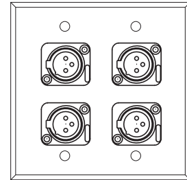
WP 2011 (4) NEUTRIK NC3FDL-1-0 "D-SERIES" 3 COND. LATCHLESS FEMALE XLR
