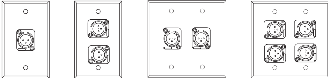
WP 1027 (1) NEUTRIK NC3MP-P "D-SERIES" 3 COND. PLASTIC MALE XLR WP 1028 (2) NEUTRIK NC3MP-P "D-SERIES" 3 COND. PLASTIC MALE XLR WP 2016 (2) NEUTRIK NC3MP-P "D-SERIES" 3 COND. PLASTIC MALE XLR WP 2018 (4) NEUTRIK NC3MP-P "D-SERIES" 3 COND. PLASTIC MALE XLR
