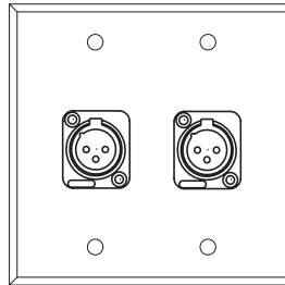
WP 2009 (2) NEUTRIK NC3FDL-1-0 "D-SERIES" 3 COND. LATCHLESS FEMALE XLR
