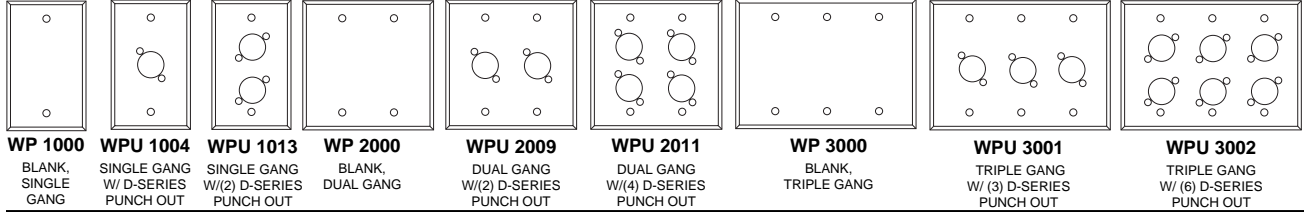
WP 1000 BLANK, SINGLE GANG WPU 1004 SINGLE GANG W/ D-SERIES PUNCH OUT WPU 1013 SINGLE GANG W/(2) D-SERIES PUNCH OUT WP 2000 BLANK, DUAL GANG WPU 2009 DUAL GANG W/(2) D-SERIES PUNCH OUT WPU 2011 DUAL GANG W/(4) D-SERIES PUNCH OUT WP 3000 BLANK, TRIPLE GANG WPU 3001 TRIPLE GANG W/ (3) D-SERIES PUNCH OUT WPU 3002 TRIPLE GANG W/ (6) D-SERIES PUNCH OUT
