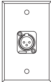
WP 1042 (1) NEUTRIK NC3FDL-1-0 "D-SERIES" 3 COND. LATCHLESS FEMALE XLR
