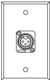
WP 1025 (1) NEUTRIK NC3FP-P "D-SERIES" 3 COND. LATCHLESS PLASTIC FEMALE XLR
