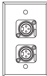
WP 1026 (2) NEUTRIK NC3FP-P "D-SERIES" 3 COND. LATCHLESS PLASTIC FEMALE XLR
