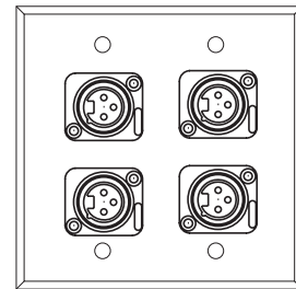
WP 1717 (4) NEUTRIK NC3FP-P "D-SERIES" 3 COND. LATCHLESS PLASTIC FEMALE XLR
