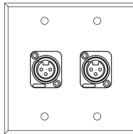
WP 1515 (2) NEUTRIK NC3FP-P "D-SERIES" 3 COND. LATCHLESS PLASTIC FEMALE XLR
