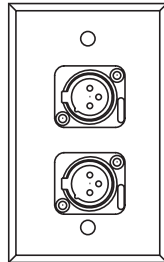
WP 1043 (2) NEUTRIK NC3FDL-1-0 "D-SERIES" 3 COND. LATCHLESS FEMALE XLR
