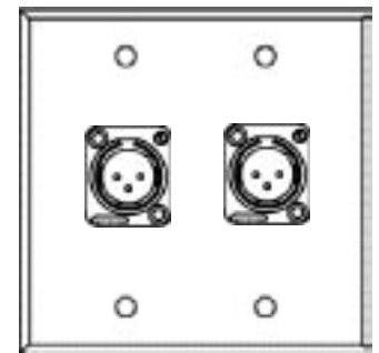
WP 2010 (2) Neutrik NC3MDL-1 "D-Series" 3 Cond. Male XLR
