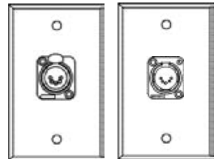
WP 1049 (1) Neutrik NC5FDL-1 "D-Series" 5 Cond. Latching Female XLR
