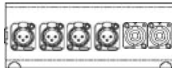
ND 6013 (4) Neutrik NC3FDL-1 "D-Series" 3 Cond. Latching Female XLR (2) Neutrik NL4MP "D-Series" 4 Cond. Speakon $84.22
