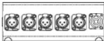
ND 6008 (5) Neutrik NC3FDL-1 "D-Series" 3 Cond. Latching Female XLR (1) Neutrik NL4MP "D-Series" 4 Cond. Speakon $83.78
