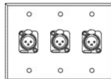
WP 3001 (3) Neutrik NC3FDL-1 "D-Series" 3 Cond. Latching Female XLR
