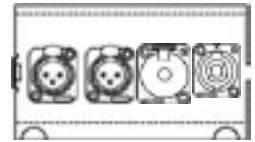
ND 4012 (2) Neutrik NC3FDL-1 Female XLR (1) Neutrik NJ3FP-6C 3 Cond. 1/4" Jack (1) Neutrik NL4MP 4 Cond. Speakon $62.68
