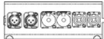
ND 6015 (2) Neutrik NC3FDL-1 "D-Series" 3 Cond. Latching Female XLR (2) Neutrik NJ3FP-6C "D-Series" 3 Cond. Locking 1/4" Jack (2) Neutrik NL4MP "D-Series" 4 Cond. Speakon $95.64
