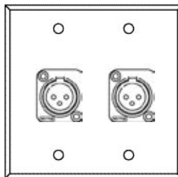
WP 2015 (2) Neutrik NC3FP-P "D-Series" 3 Cond. Latchless Plastic Female XLR
