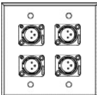
WP 2012 (4) Neutrik NC3MDL-1 "D-Series" 3 Cond. Male XLR
