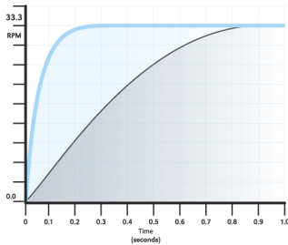
Numark TTX1 Start Time vs. Industry Standard
