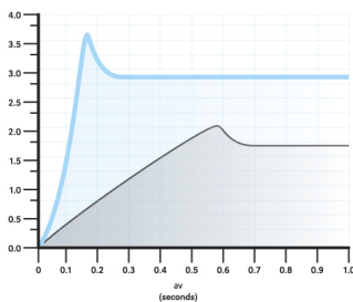
Numark TTX1 Torque vs. Industry Standard
