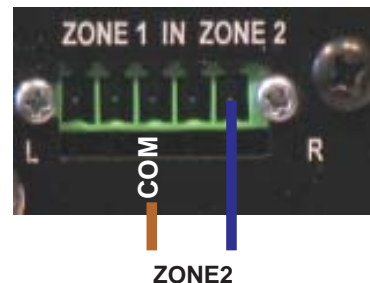
ZONE2 SINGLE ZONE MODE
