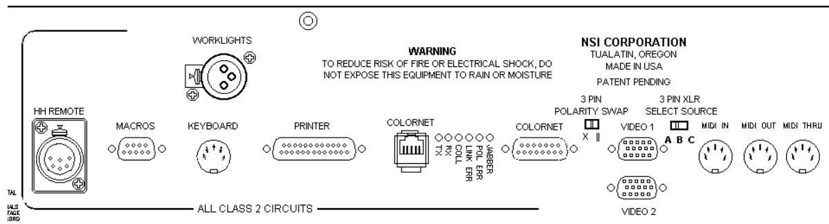
FIGURE 1.4 MONITOR AND PERIPHERAL DEVICE CONNECTIONS
