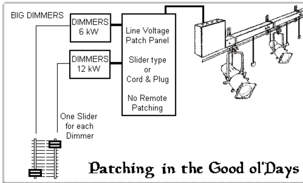
FIGURE 5.1A LIGHTING CONTROL OLD PATCH FUNCTIONAL DIAGRAM
