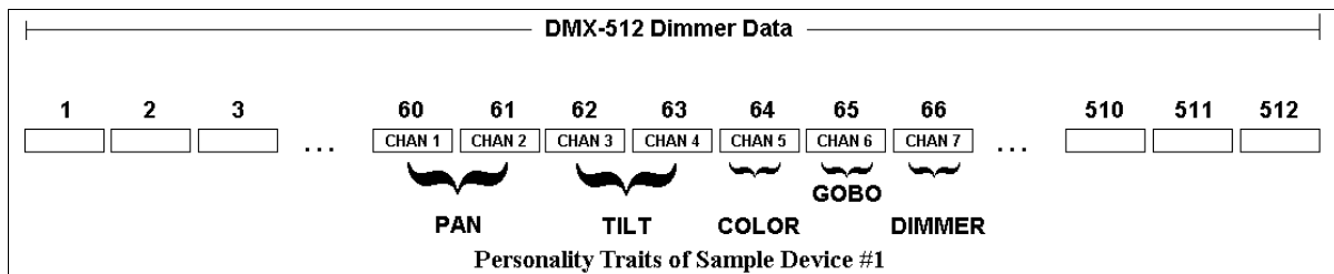
FIGURE 23.1 ILLUSTRATION OF SAMPLE MOVING LIGHTING TRAITS AND THE RELATIONSHIP TO DMX
