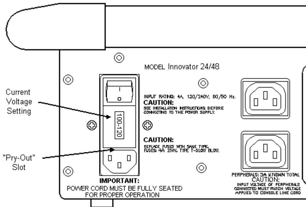
FIGURE 1.1 INNOVATOR POWER CONNECTIONS
