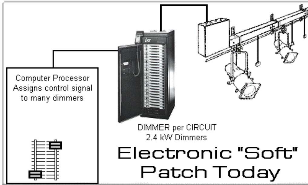
FIGURE 5.1B LIGHTING CONTROL SYSTEM PATCH FUNCTIONAL DIAGRAM
