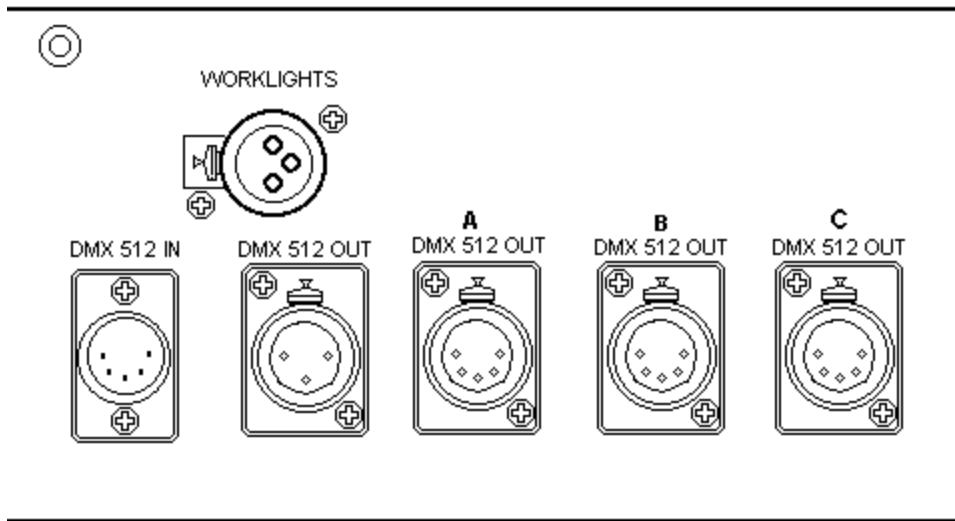
FIGURE 1.3 - INNOVATOR DIMMER CONNECTIONS
