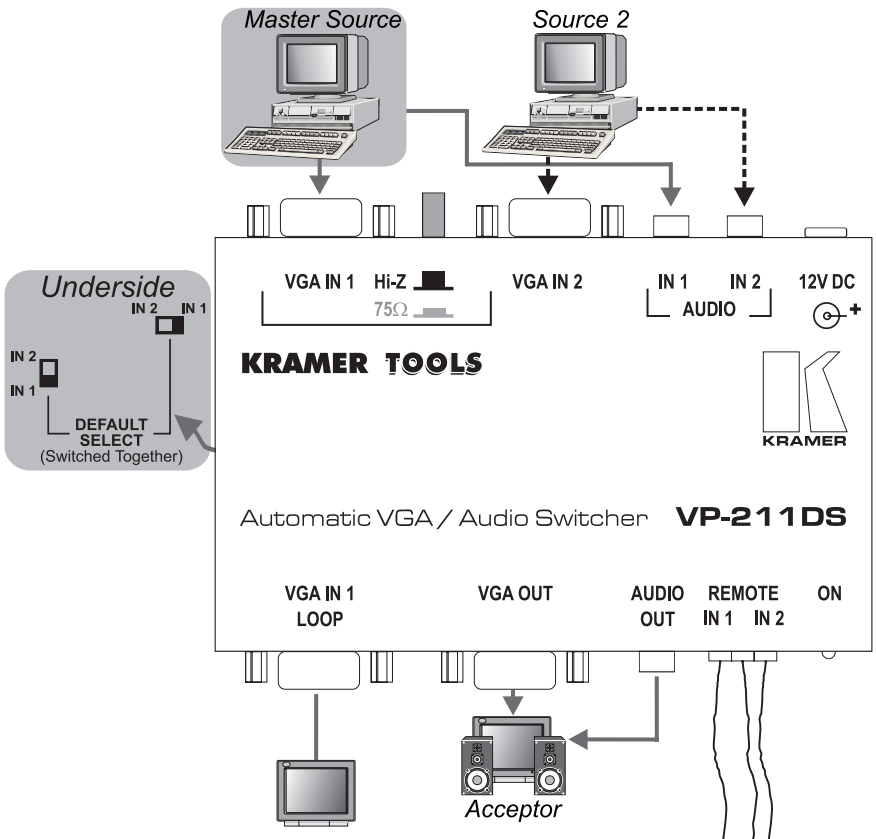
Additional Monitor Release the loop termination switch (Hi-Z) Connect to a Dry Contact Switch
