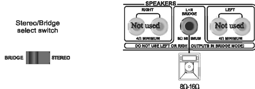
BRIDGE connection
