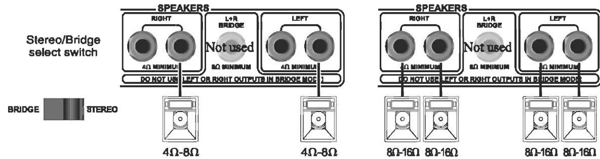
Two-channel connection
