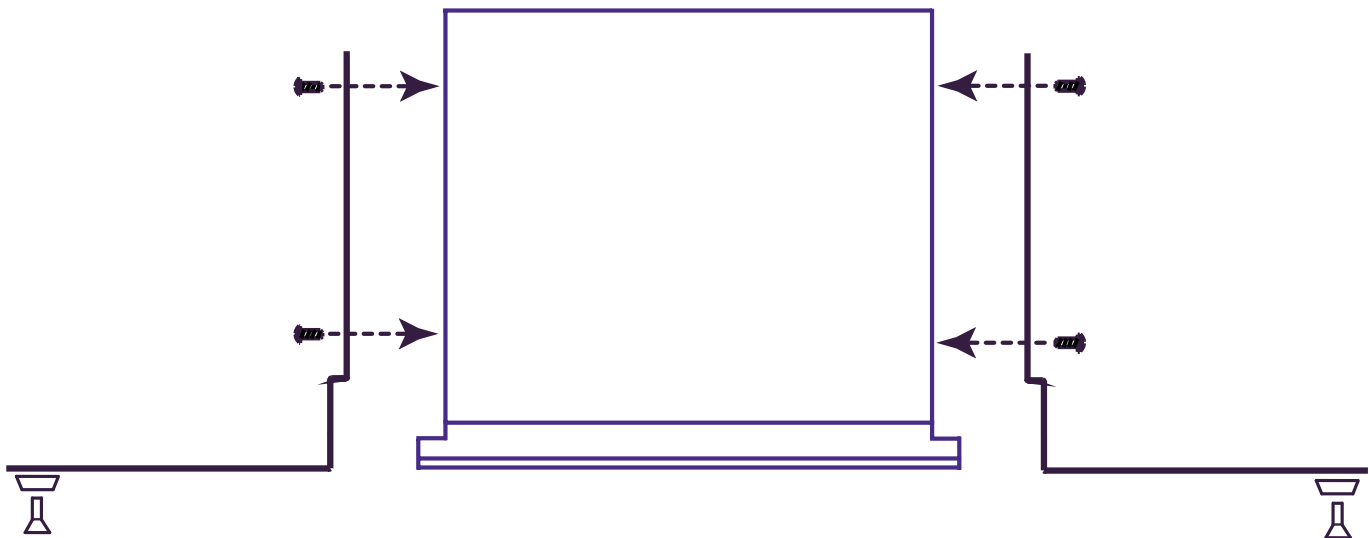
Rack mount ear positioning (top view)
