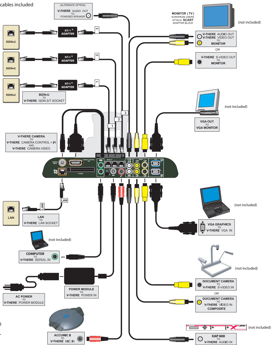
V-There connection diagram.
