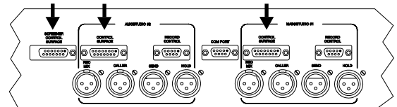
Figure 6. Serial cable mainframe attachment.
