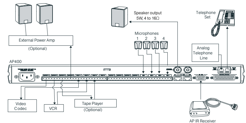
Figure 3. An AP IR receiver connected to an AP400 system
