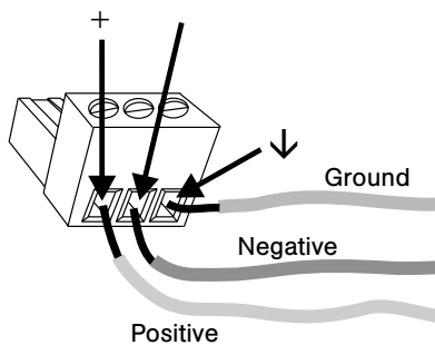
Figure 7. Phoenix push-on connector
