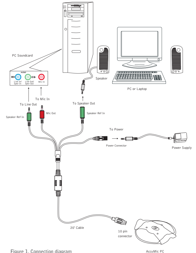
Figure 1. Connection diagram
