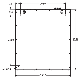
TOP VIEW (SL-236SP)
