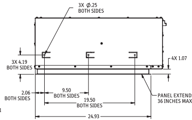
SIDE VIEW (SL-236SP)
