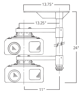
Front View (LCD-2C Ceiling Plate)
