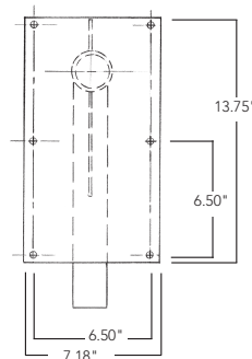
Top View (LCD-2C Ceiling Plate)
