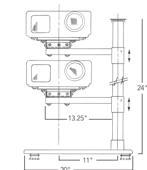
Front View (LCD-2TS Table Stand)
