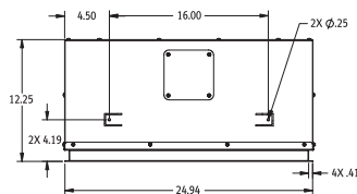
FRONT VIEW (SL-236SP)
