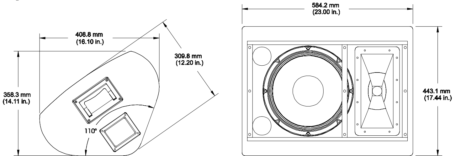
Figure 8—Dimensions
