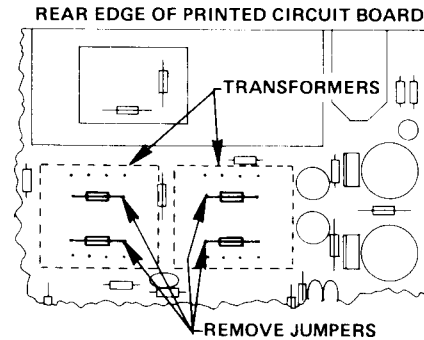
FIGURE 9 - Mounting Location of Optional TRB-1 Transformers
