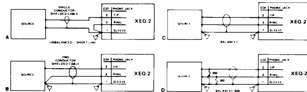
FIGURE 8 - Input Connections to the XEQ-2
