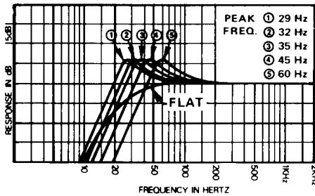
FIGURE 3 - Low-Frequency Equalization
