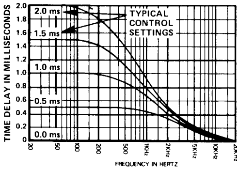
FIGURE 4 - Low-Frequency Time Delay
