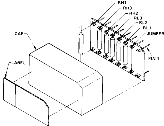
FIGURE 7 - Crossover Module Assembly
