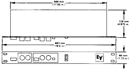
FIGURE 1 - Dimensions
