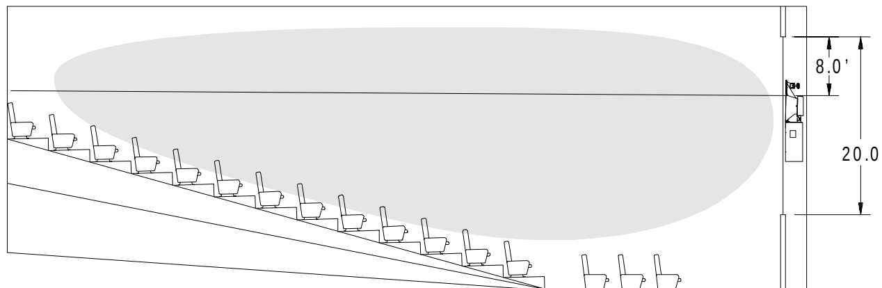
Figure 2—Aiming the Variplex™-B
