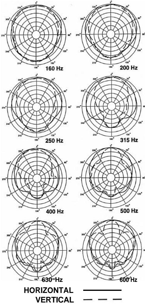
FIGURE 2 - TL606DW One-Third-Octave Polar Responses (anechoic environment)
