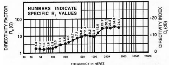
FIGURE 4 - TL606DW Directivity vs Frequency Whole Space (anechoic)
