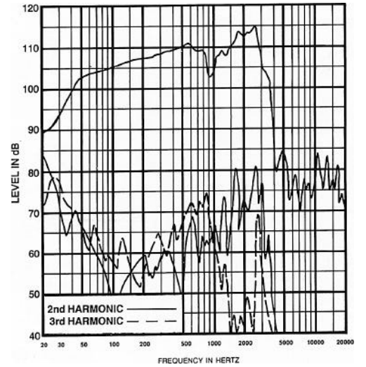
FIGURE 6 - TL606DW Harmonic Distortion, 0.1 Rated Power Input (60 watts), 10 Feet on Axis
