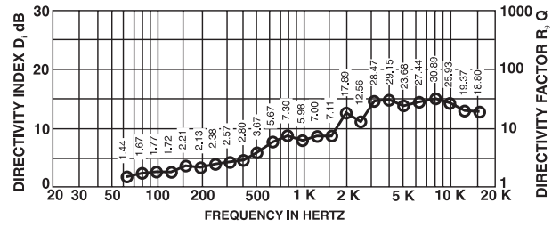
FIGURE 4 — T221 Directivity vs. Frequency, Whole Space (anechoic)
