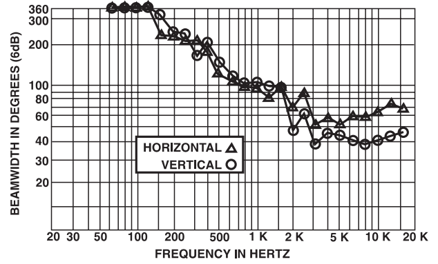
FIGURE 3 — T221 Beamwidth vs. Frequency, Whole Space (anechoic)
