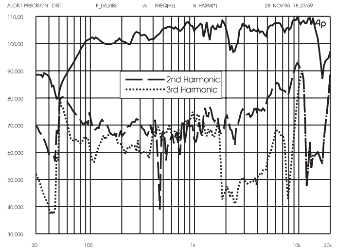
FIGURE 5 — T221 Distortion at 40 watts
