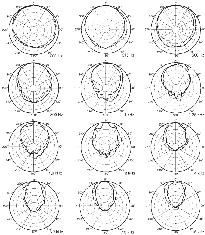
FIGURE 1 — T221 Polar Response (one-third-octave pink noise)
