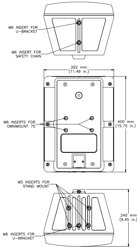
Figure 8— Sx80T enclosure with Sx80SM stand mounting kit.
