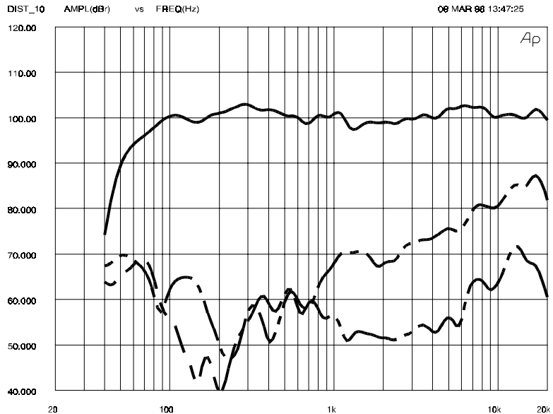
Figure 5 — Harmonic Distortion Response 10% Rated Power Input (40 watts), (anechoic environment, 3.05 meters (10 feet), on axis)
