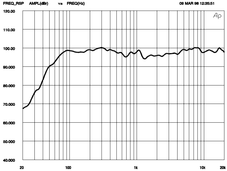
Figure 1a—Axial Frequency Response, (anechoic environment, 4 volts/3.05 meters (10 feet), normalized to 1 watt/1 meter) (open ports)
