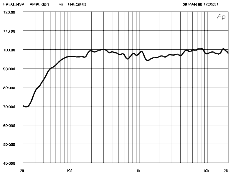
Figure 1b—Axial Frequency Response, (anechoic environment, 4 volts/3.05 meters (10 feet), normalized to 1 watt/1 meter) (closed ports)
