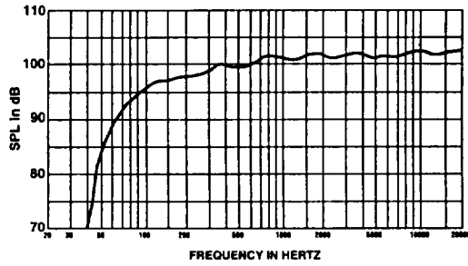
FIGURE 1 — Sx200a Frequency Response (1 watt/1 meter, anechoic environment)
