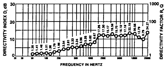
FIGURE 6 — Sx200a Directivity Response (anechoic environment)
