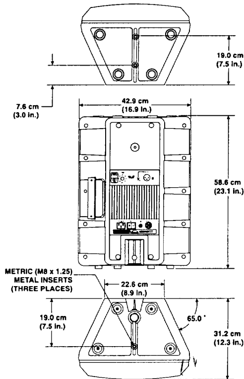
FIGURE 2 — Sx200a Dimensions
