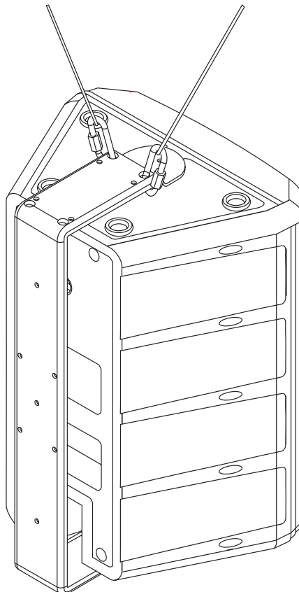
FIGURE 4 — Suspending the S b 121a Using the M b 200 Installation Kit
