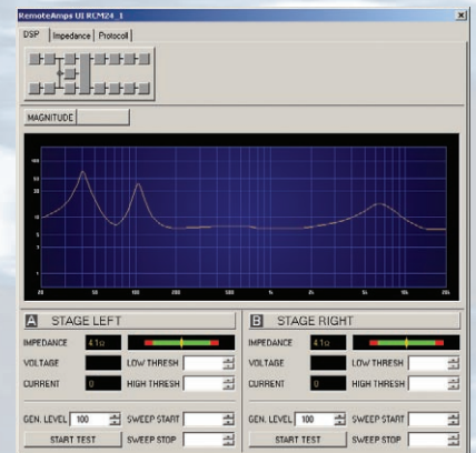
Supervision for each connected loudspeaker with individual upper and lower thresholds for impedance values. An out-of-limit device will show up immediately.
