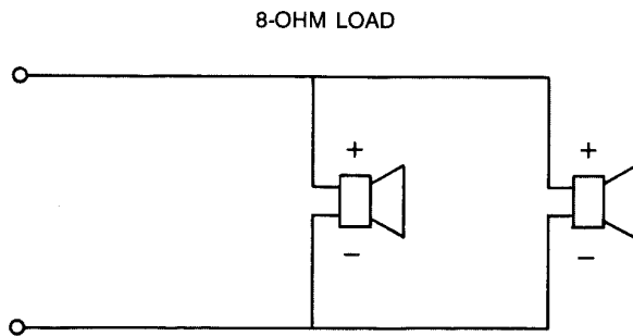
FIGURE 8 Electrical Connections
