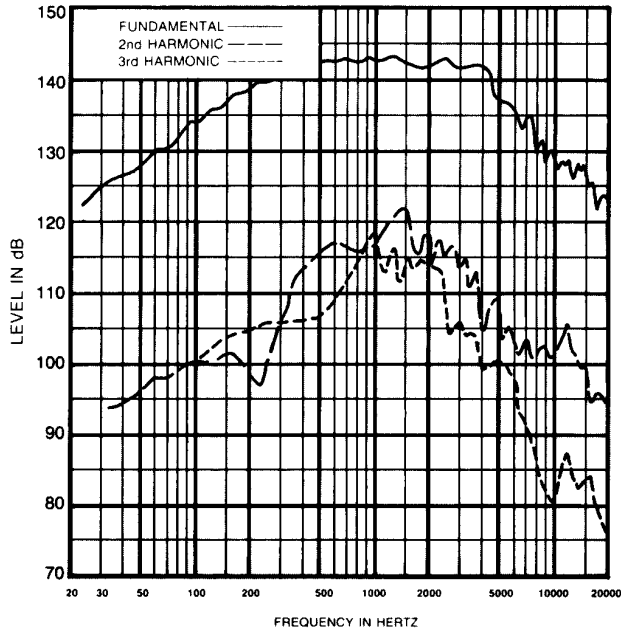
FIGURE 4 Distortion Response, 2-Inch Plane-Wave Tube, 10 Watts
