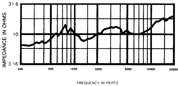
FIGURE 6 Impedance Response — 2-Inch Plane-Wave Tube
