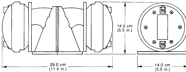
FIGURE 2 Dimensions
